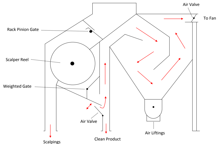
Scalper Aspirator Cross Section
